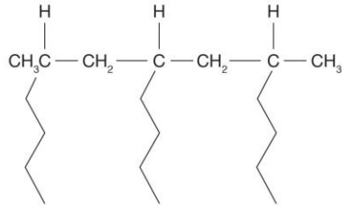
Figure 1 - Sample of chemical structure of PAO
