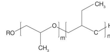
Figure 2 - Sample of chemical structure of PAG
